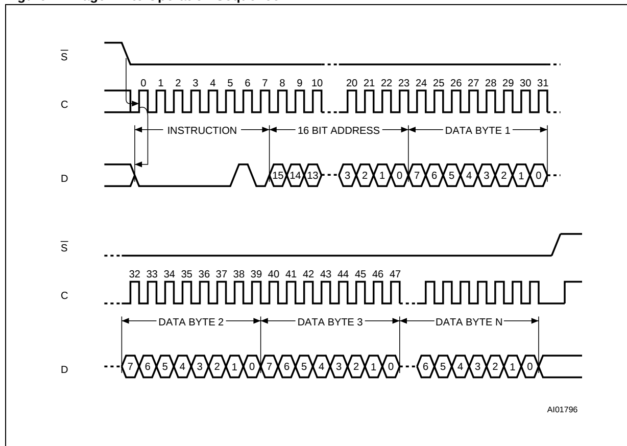
Figure 12. Page Write Operation Sequence
