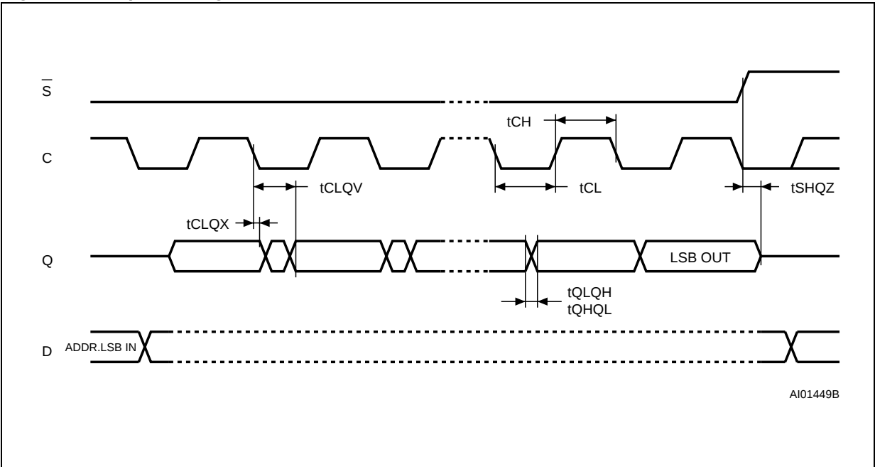
Figure 15. Output Timing
