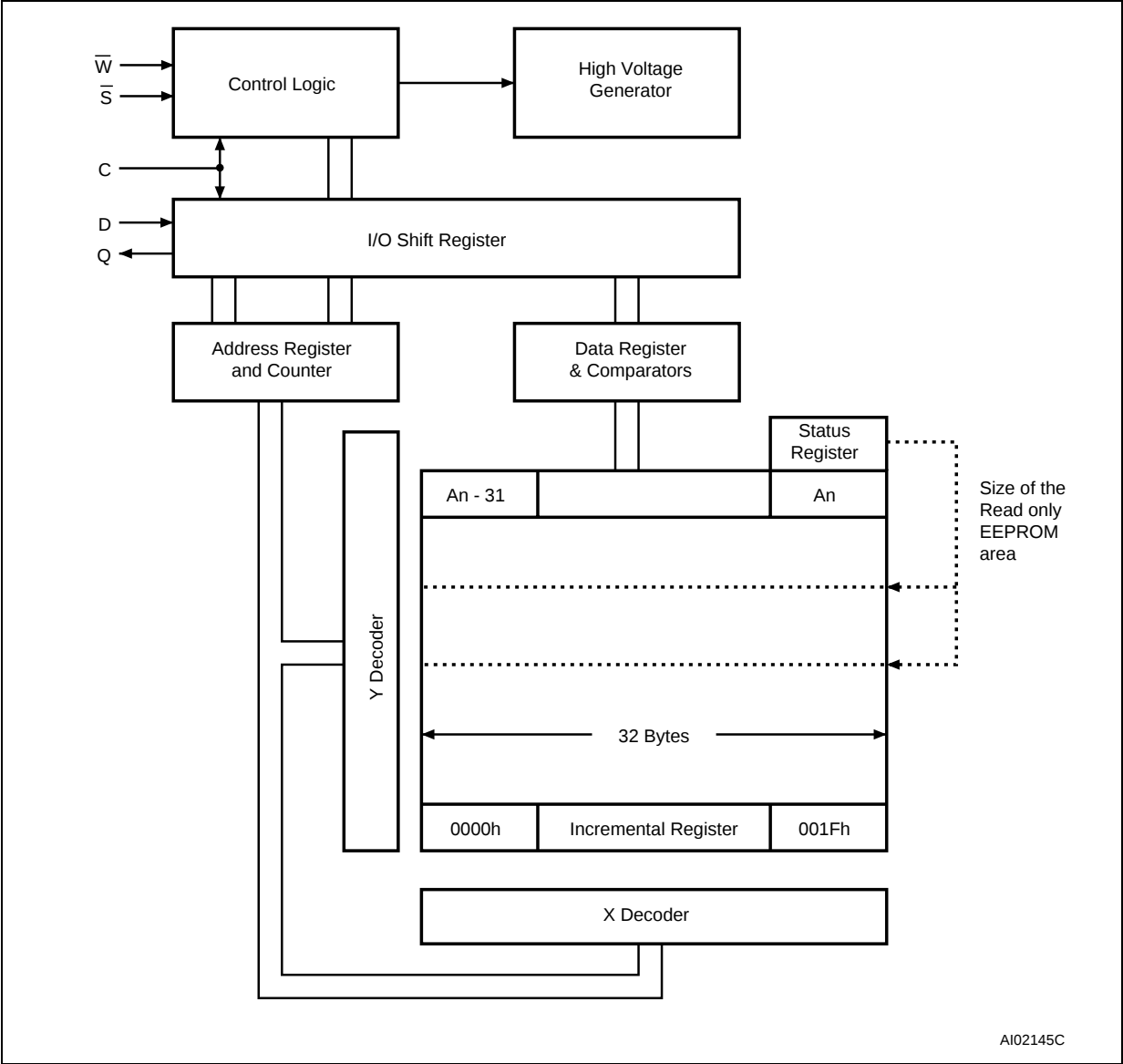
Figure 11. Block Diagram
